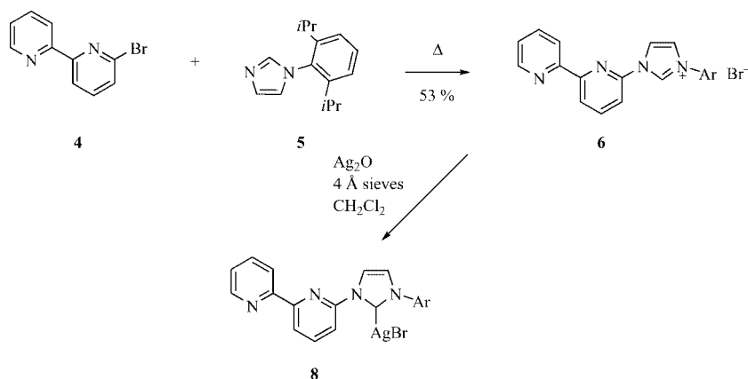
Scheme 3. Formation of the “bipy” salt 6 and attempt to deprotonate (Ar = 2,6- i Pr 2 C 6 H 3 ).
