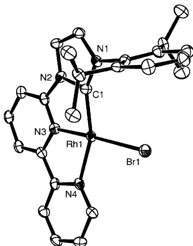
Figure 4. ORTEP representation of the structure of 9a showing 50% probability ellipsoids with hydrogen atoms omitted for clarity. Selected bond lengths [Å] and angles [°] with estimated standard deviations: C(1)–Rh(1) 1.957(6), N(3)–Rh(1) 1.941(5), N(4)–Rh(1) 2.116(5), Br(1)–Rh(1) 2.4904(8); N(3)–Rh(1)–Br(1) 172.26(14), C(1)–Rh(1)–Br(1) 104.30(17), N(4)–Rh(1)–Br(1) 97.27(13).
