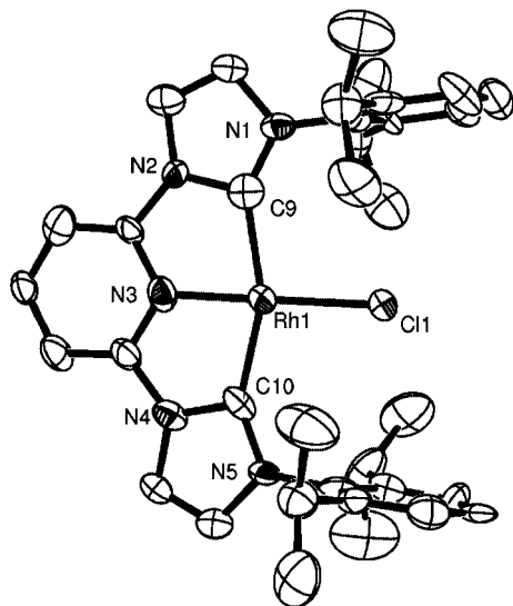
Figure 1. ORTEP representation of the structure of 2 showing 50% probability ellipsoids with hydrogen atoms omitted for clarity. Selected bond lengths [Å] and angles [°] with estimated standard deviations: Rh(1)–Cl(1) 2.331(3), Rh(1)–N(3) 1.955(8), Rh(1)–C(9) 2.001(10), Rh(1)–C(10) 1.979(9); N(3)–Rh(1)–Cl(1) 178.4(3), N(3)–Rh(1)–C(9) 78.5(4), N(3)–Rh(1)–C(10) 79.4(4), C(9)–Rh(1)–Cl(1) 101.2(3), C(10)–Rh(1)–Cl(1) 100.8(3).
