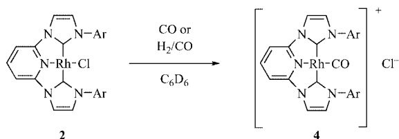
Scheme 2. Reaction of complex 2 with CO (Ar = 2,6- i Pr _2 C _6 H _3 ).
