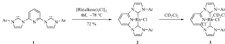
Scheme 1. Synthesis of rhodium complexes 2 and 3 (alkene = C 2 H 4 , C 8 H 14 ; Ar = 2,6- i Pr 2 C 6 H 3 ).
