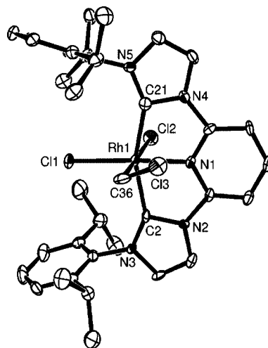
Figure 2. ORTEP representation of the structure of 3 showing 50% probability ellipsoids with hydrogen atoms and one molecule of \text{CD}_2\text{Cl}_2 omitted for clarity. Selected bond lengths [Å] and angles [°] with estimated standard deviations: Rh(1)–Cl(1) 2.3656(15), Rh(1)–Cl(2) 2.5164(16), Rh(1)–C(36) 2.075(6), Rh(1)–N(1) 1.978(4), Rh(1)–C(21) 2.034(6), Rh(1)–C(2) 2.040(6); N(1)–Rh(1)–Cl(1) 177.68(15), N(1)–Rh(1)–C(21) 79.1(2), N(1)–Rh(1)–C(2) 79.2(2), C(36)–Rh(1)–Cl(2) 177.22(19).
