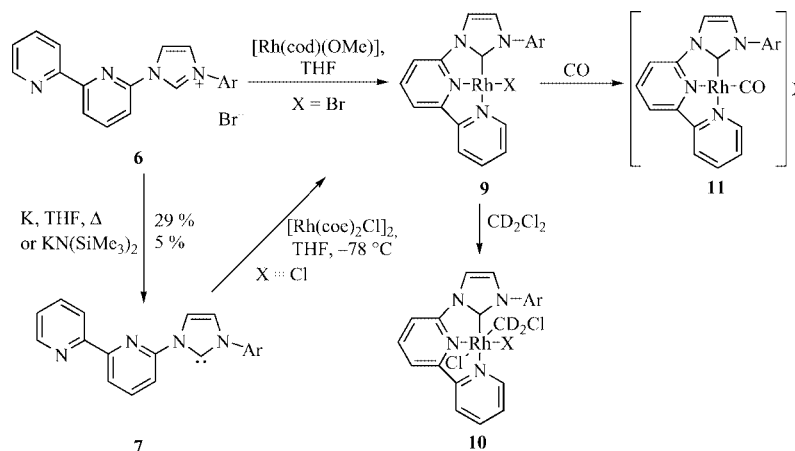
Scheme 4. Generation of free carbene 7 and complexes 9a and 9b (Ar = 2,6- i Pr 2 C 6 H 3 ; 9a : X = Br; 9b : X = Cl).
