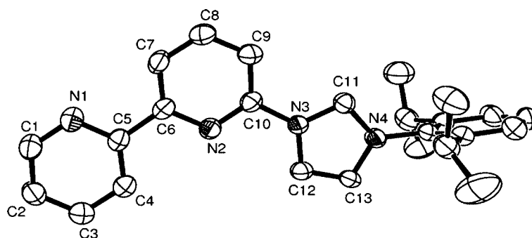
Figure 3. ORTEP representation of the structure of 7 showing 50% probability ellipsoids with hydrogen atoms omitted for clarity. Selected bond lengths [Å] and angles [°] with estimated standard deviations: C(11)–N(4) 1.361(3), C(11)–N(3) 1.375(3), C(5)–C(6) 1.486(4), C(10)–N(3) 1.427(3); N(4)–C(11)–N(3) 101.3(2).
